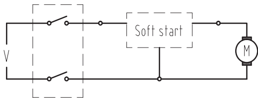
electrical diagram
